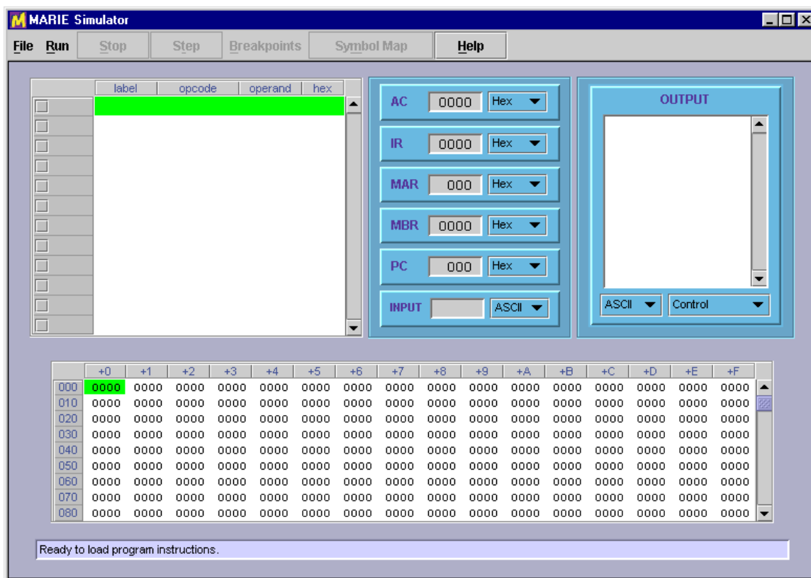
Figure 1: The MarieSim Graphical Environment
